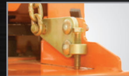
Patented deck-leveling adjustment is quick and easy — select zero-turn riders.
