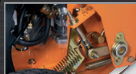
SWZ: Adjust-A-Trac tool is conveniently mounted on the engine deck for quick and easy neutral and tracking adjustments in the field.
